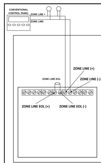
Picture 11 - Conventional line wiring (zone line EOL resistor inside of the device)
