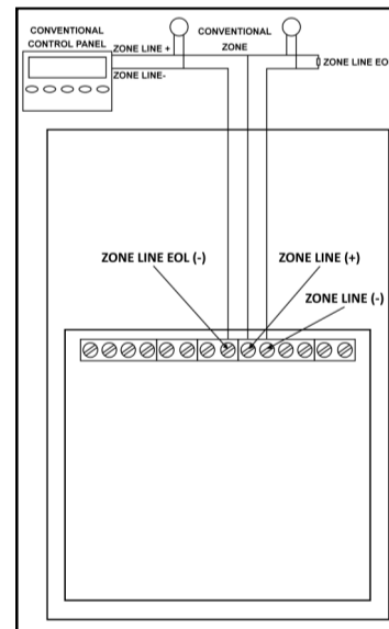
Picture 10 - Conventional line wiring (zone line EOL resistor outside of the device)
