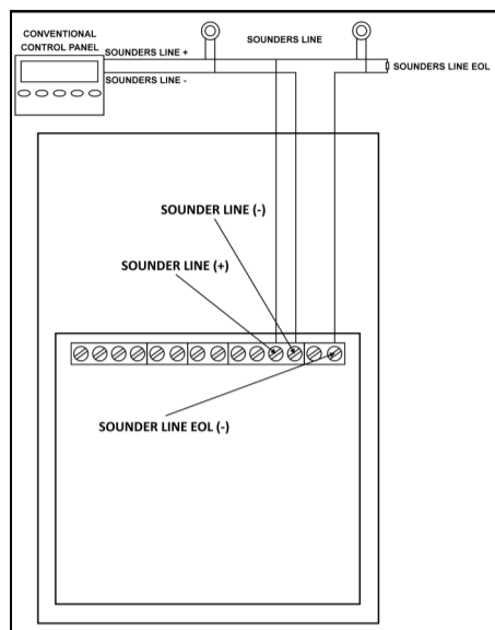
Picture 12 - Sounders line wiring (sounders line EOL resistor outside of the device)
